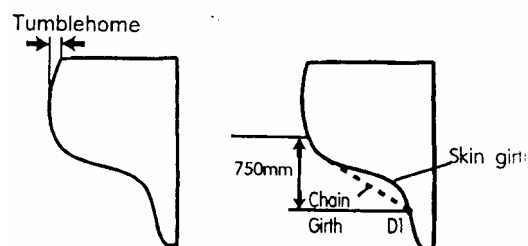
Midship cross-section at 0.55 x LWL from forward end of LWL
